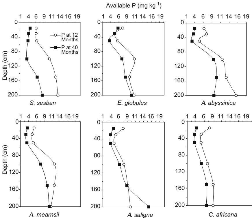
Figure 4. Trends of available P at 12 and 40 months under different trees on a Vertisol area of Ginchi, central Ethiopia.
