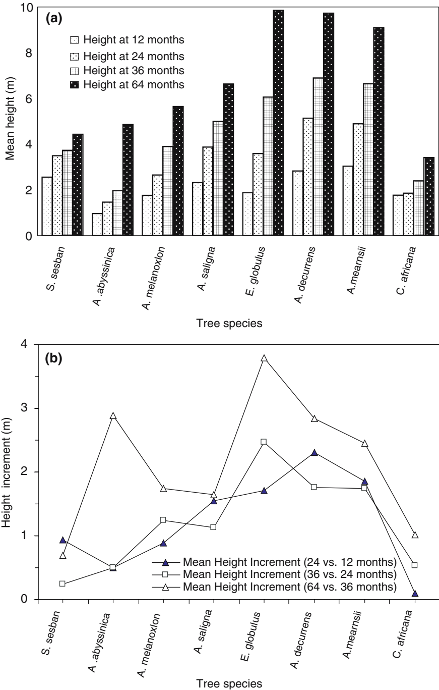
Figure 2. Tree species evaluated on a Vertisol area of Ginchi, central Ethiopia (a) mean height and (b) mean height increment.
